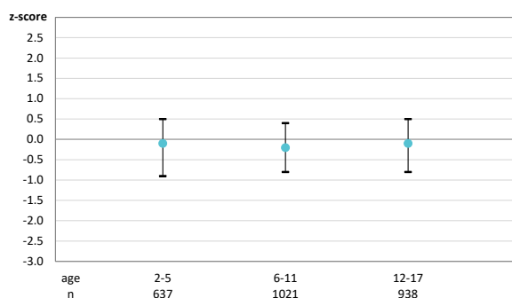
Quartiles of z-scores for BMI: Germany
