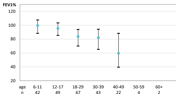
Quartiles of FEV 1 %: Slovak Republic
