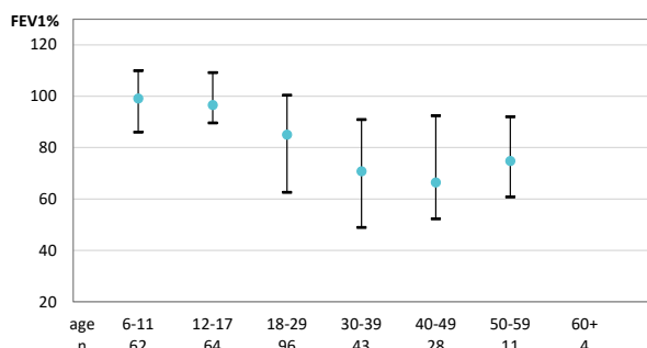
Quartiles of FEV 1 %: Russian Federation
